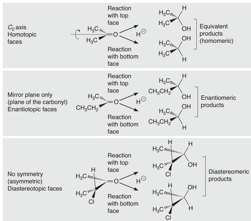
Figure 6.7 Stereochemical consequences of reacting three different types of carbonyls with a hydride reducing agent.
